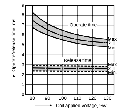
3-(5). Operate/release time Sample: JW2SN-DC12V, 6 pcs. Ambient temperature: 20°C 68°F
