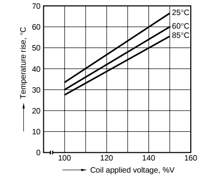
4-(1). Coil temperature rise (Contact carrying current: 5A) Sample JW1aFSN-DC12V, 6 pcs. Point measured: Inside the coil
