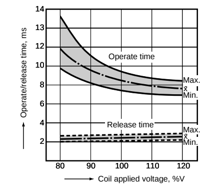
3-(4). Operate/release time Sample: JW2aSN-DC24V, 6 pcs. Ambient temperature: 20°C 68°F
